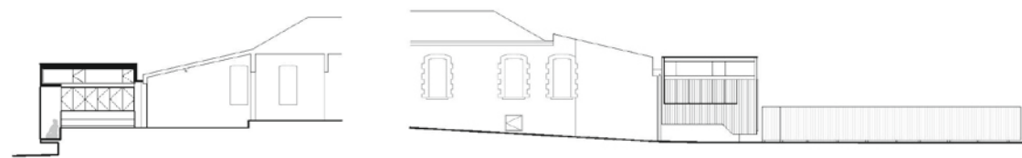
BELLEVUE TERRACE ALTERATIONS + ADDITIONS 0 1 3 6M LONGITUDINAL SECTION SCALE: 1:200 @ A4
